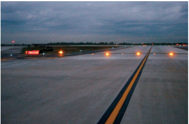
Runway holding position as viewed from a taxiway centerline. This holding position has both above ground and in-pavement runway guard lights.
